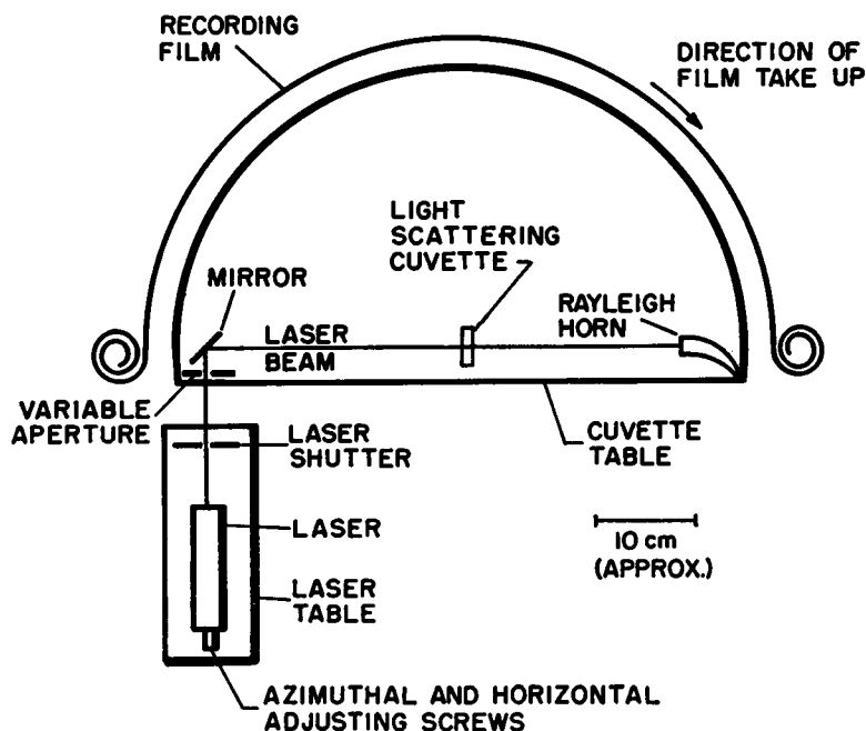
FIGURE 3 Schematic diagram of the film photometer. The laser provides incident light to the scatterers in the cuvette. Most of the laser light is dumped into the Rayleigh horn while the film records the scattered light.
